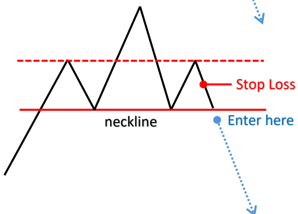
Head & Shoulders
