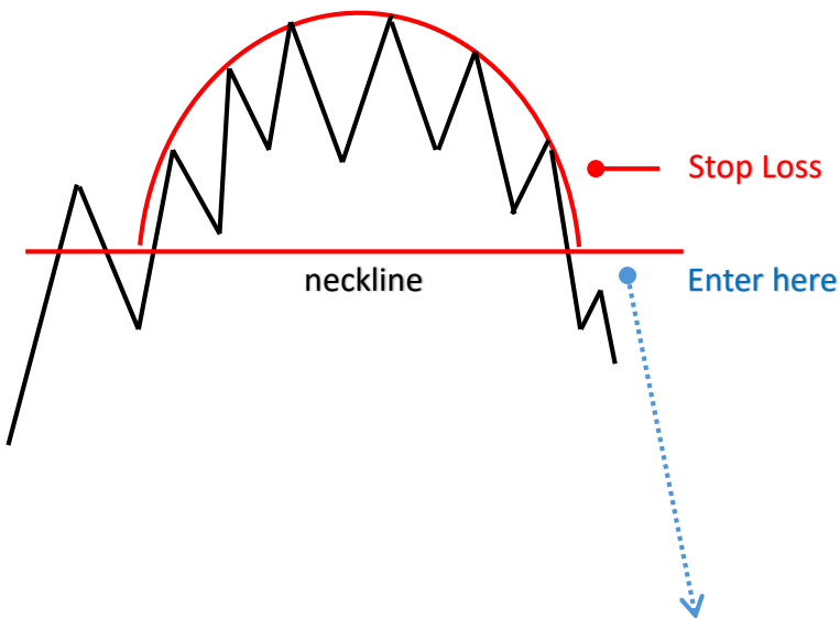
Rounding Top
