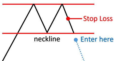
Double Top
